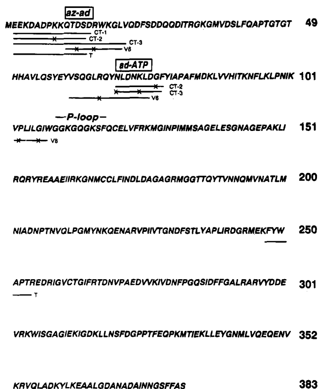
FIGURE 9: Positions of photolabeled peptides in the primary sequence of tobacco Rubisco activase. The figure includes the data for peptides recovered after digestion of photolabeled Rubisco activase with chymotrypsin (CT), trypsin (T), and V8 protease (V8). CT-1, CT-2, and CT-3 refer to chymotryptic peptides recovered after photoaffinity labeling with 2-N 3 ATP in the presence of ADP and Trp (Table 2) or in the absence of effector, respectively. Assignment of the adenine binding domain for ATP (ad-ATP) and the azidoadenine nucleotide domain (az-ad) was based on selective protection of these peptides by ADP and Trp.
