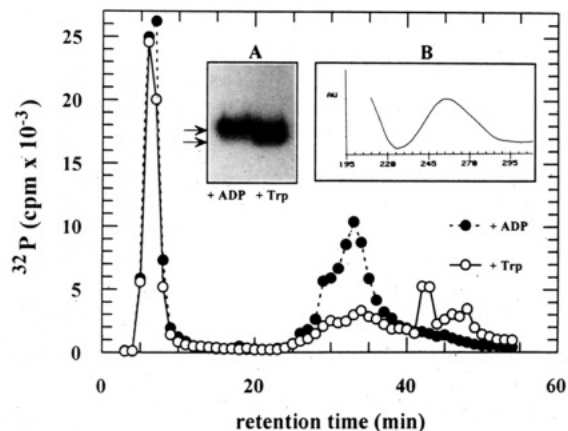
FIGURE 8: Separation of photolabeled peptides from Rubisco activase by reverse-phase HPLC. Rubisco activase (0.5 mg) was photoaffinity labeled with 50 \mu\text{M} [\gamma\text{-}^{32}\text{P}]\text{2-N}_3\text{ATP} in the presence of 300 \mu\text{M} ADP or 150 \mu\text{M} Trp in a total volume of 0.5 mL. After precipitation with saturated ammonium sulfate and desalting, aliquots of the desalted protein were subjected to SDS-PAGE. The remainder was digested with chymotrypsin, and photolabeled peptides were affinity purified on an \text{Al}^{3+} -chelate column and then separated by reverse-phase HPLC. (Inset A) Autoradiogram of Rubisco activase polypeptides, separated by SDS-PAGE, after photoaffinity labeling with [\gamma\text{-}^{32}\text{P}]\text{2-N}_3\text{ATP} in the presence of ADP or Trp. The main figure shows the ^{32}\text{P} profile of the reverse-phase HPLC separation of \text{Al}^{3+} -chelate chromatography-purified photolabeled peptides from Rubisco activase photoaffinity labeled with [\gamma\text{-}^{32}\text{P}]\text{2-N}_3\text{ATP} in the presence of ADP (●) or Trp (○). (Inset B) The ultraviolet spectra of the peptide peak corresponding to the radioactive peak at 33 min in the chromatogram (●).
