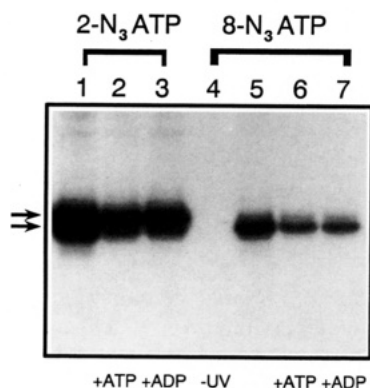
FIGURE 3: Effect of ATP and ADP on photoaffinity labeling of recombinant tobacco Rubisco activase with [\gamma\text{-}^{32}\text{P}]2\text{-N}_3\text{ATP} . Autoradiogram of Rubisco activase polypeptides, separated by SDS-PAGE, after incubation and photolysis with 10\text{ }\mu\text{M} [\gamma\text{-}^{32}\text{P}]2\text{-N}_3\text{ATP} (lanes 1–3) or 8\text{-N}_3\text{ATP} (5–7) in the absence (lanes 1 and 5) and presence of 300\text{ }\mu\text{M} ATP (lanes 2 and 6) or ADP (lanes 3 and 7). In lane 4, Rubisco activase was incubated with [\gamma\text{-}^{32}\text{P}]8\text{-N}_3\text{ATP} but not photolyzed. The arrows indicate the positions of the two radiolabeled bands at 42 and 44 kDa.
