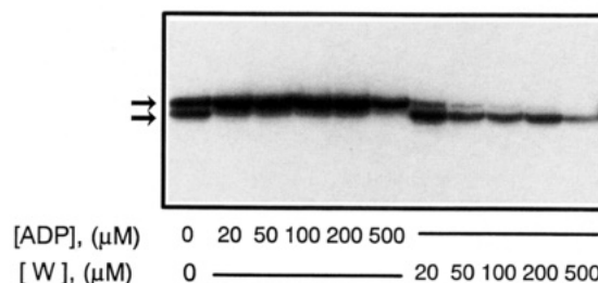
FIGURE 4: Effect of ADP and Trp concentration on photoaffinity labeling of recombinant tobacco Rubisco activase with [\gamma\text{-}^{32}\text{P}]2\text{-N}_3\text{ATP} . Autoradiogram of Rubisco activase polypeptides, separated by SDS-PAGE, after incubation and photolysis with 10\text{ }\mu\text{M} [\gamma\text{-}^{32}\text{P}]2\text{-N}_3\text{ATP} in the absence (lane 1) or presence of the indicated concentrations of Trp (lanes 2–6) or ADP (lanes 7–11). The arrows indicate the positions of the two radiolabeled bands at 42 and 44 kDa.
